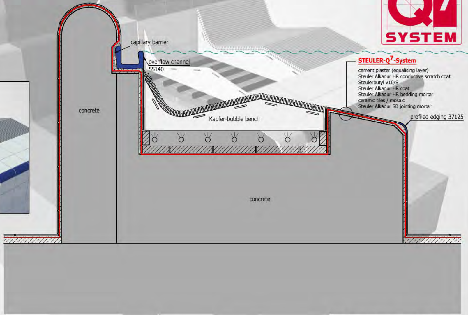
sectional drawing 9.3 bubble bench
