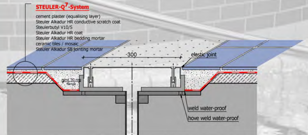
sectional drawing 9.2 sparkling-plate e.g. Fluvo
