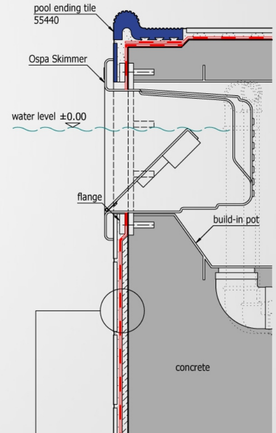
sectional drawing 6.1 skimmer
